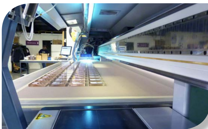
Coasters are held securely on a vacuum table during printing. Hundreds of parts are printed at the same time for maximum cost efficiency.
